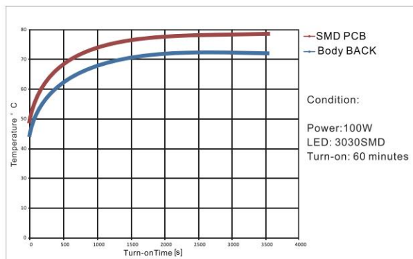
Temperature Rise
