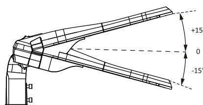
Vertical Installation ±0-5-10-15°
